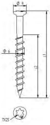
Eurofast GBS-A2 6,0 x L
